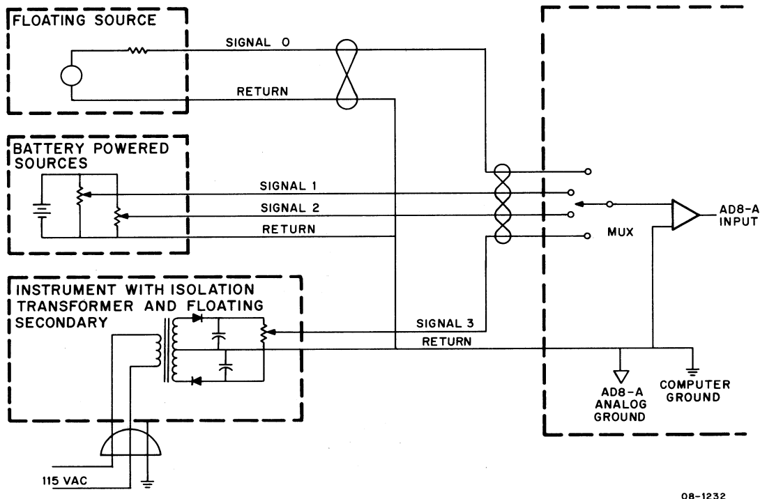
Figure 2-2 Floating AD8-A Input Signals
