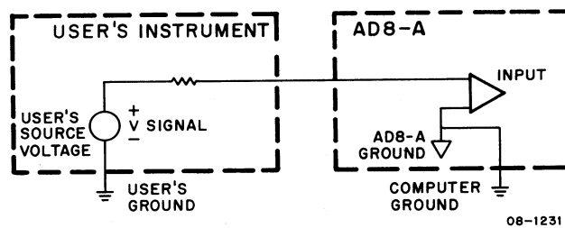
Figure 2-1 AD8-A Input Referenced to User's Ground
