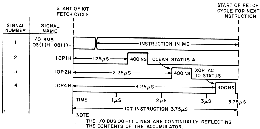
Figure 3-5B Command Register Timing with PDP-8
