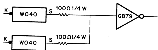
Figure 6-6 G879 Application
